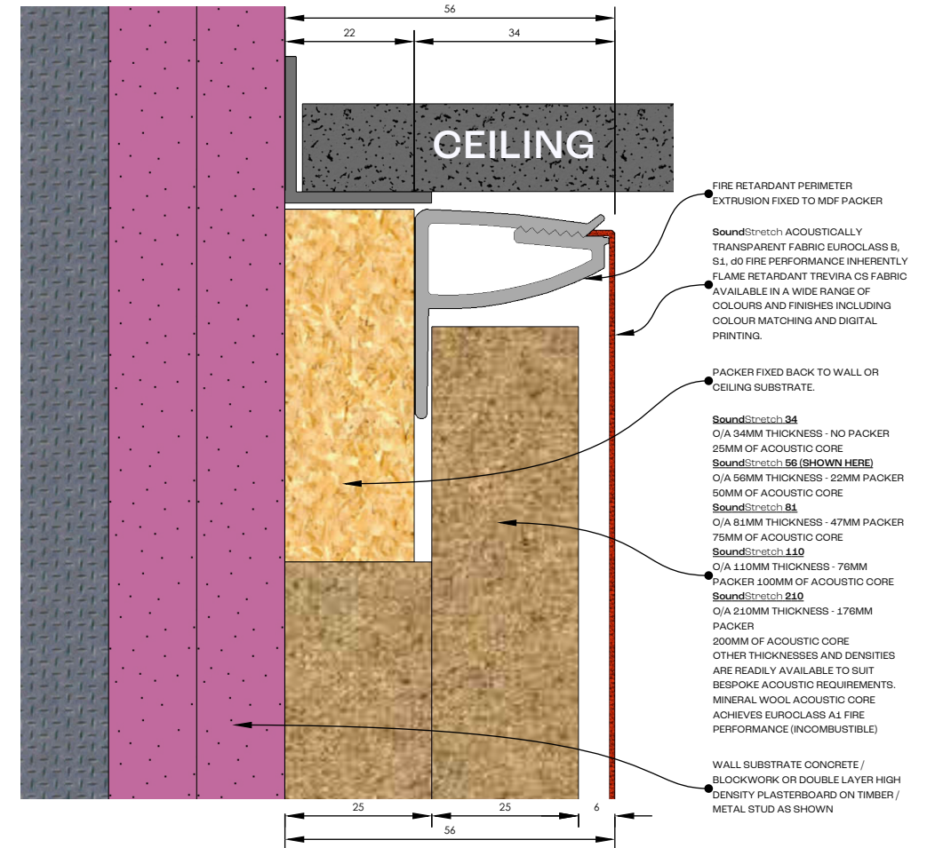
B :: SOUNDSTRETCH 56 | SECTION THRU PANEL @ CEILING
